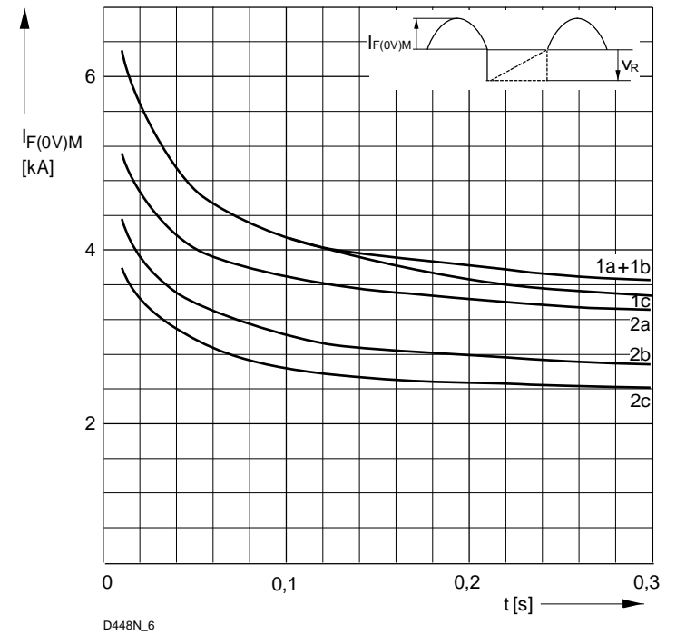
Bild / Fig. 4 Grenzstrom / Maximum overload forward current I_{F(OV)M} = f(t) 1 - I_{FAV(vor)} = 0\text{ A} ; t_{vj} = t_c = 25\text{ °C} 2 - I_{FAV(vor)} = 450\text{ A} ; t_c = 122\text{ °C} ; t_{vj} = 180\text{ °C} a - V_R \leq 50\text{ V} b - V_R = 0,5 V_{RRM} c - V_R = 0,8 V_{RRM}
