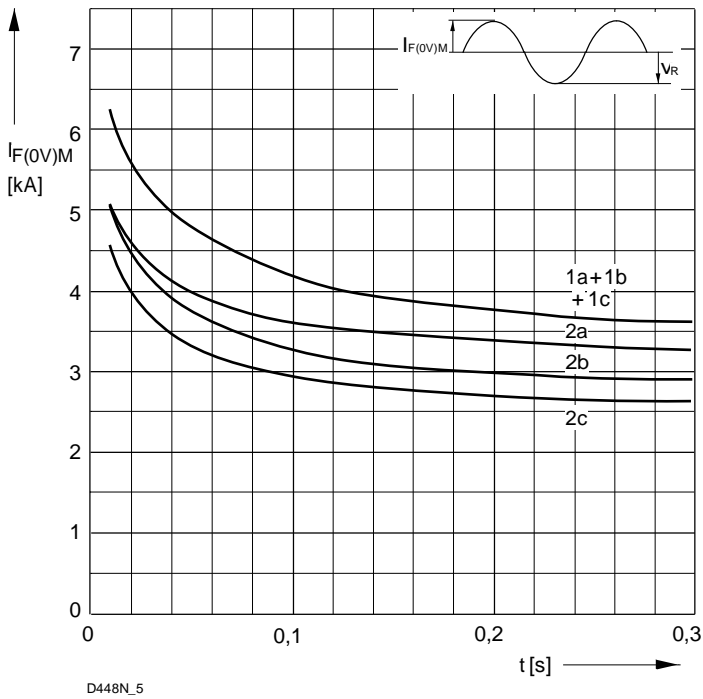
Bild / Fig. 3 Grenzstrom / Maximum overload forward current I_{F(OV)M} = f(t) 1 - I_{FAV(vor)} = 0\text{ A} ; t_{vj} = t_c = 25\text{ °C} 2 - I_{FAV(vor)} = 450\text{ A} ; t_c = 122\text{ °C} ; t_{vj} = 180\text{ °C} a - V_R \leq 50\text{ V} b - V_R = 0,5 V_{RRM} c - V_R = 0,8 V_{RRM}
